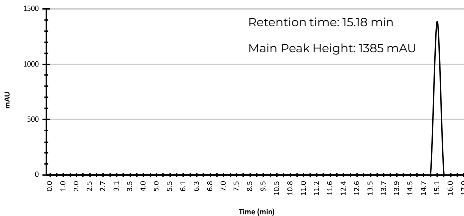
HPLC Chromatogram
