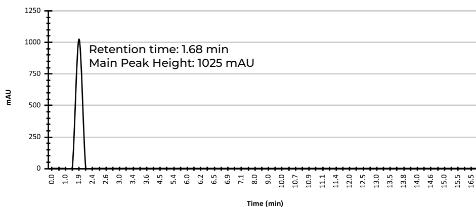
HPLC Chromatogram
