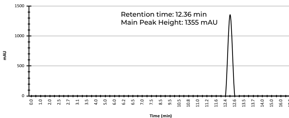
HPLC Chromatogram
