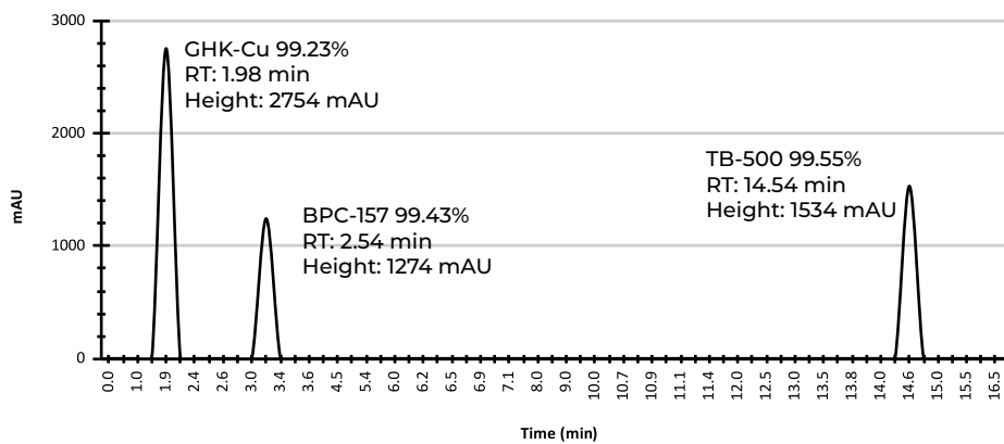
HPLC Chromatogram
